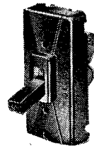
2 T 10A 250 V D.P. Panel mounting, also S.P. 2-way and momentary contact
