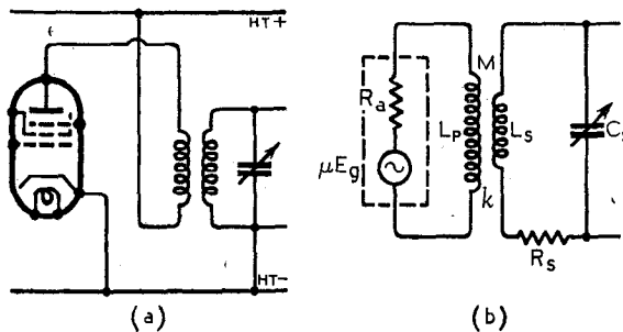
Fig. 2. An RF transformer may also be considered as a matching circuit. The circuit diagram of such a stage is given at (a) and its electrical equivalent at (b).
