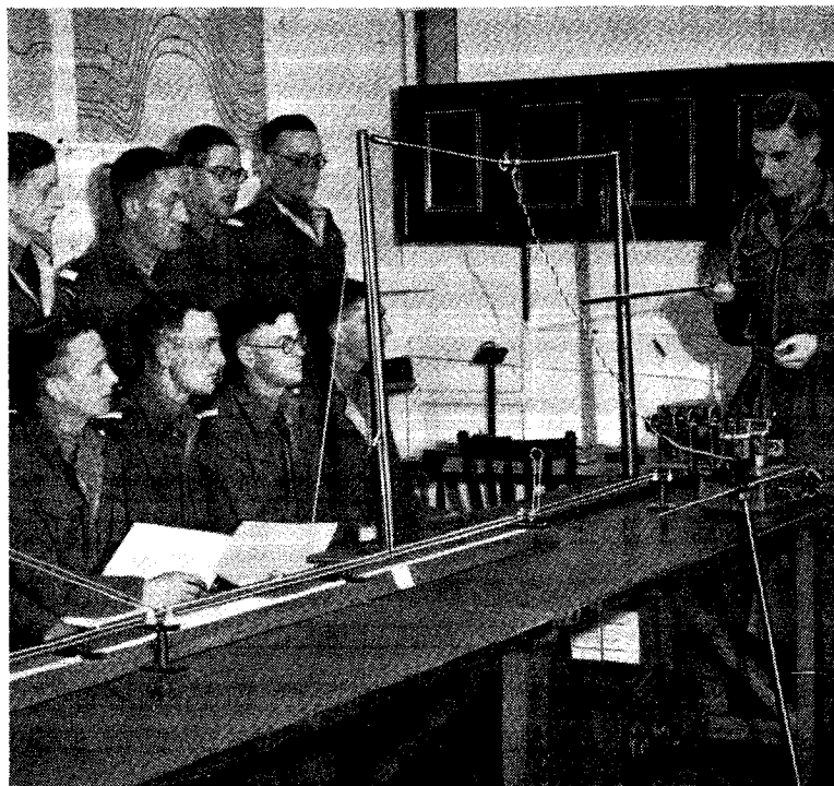
Aerial Demonstration Room. Cadets being instructed in the use of a twisted-pair feeder to a half-wave aerial.
