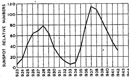
Fig. 1. Annual means of relative sunspot numbers.
